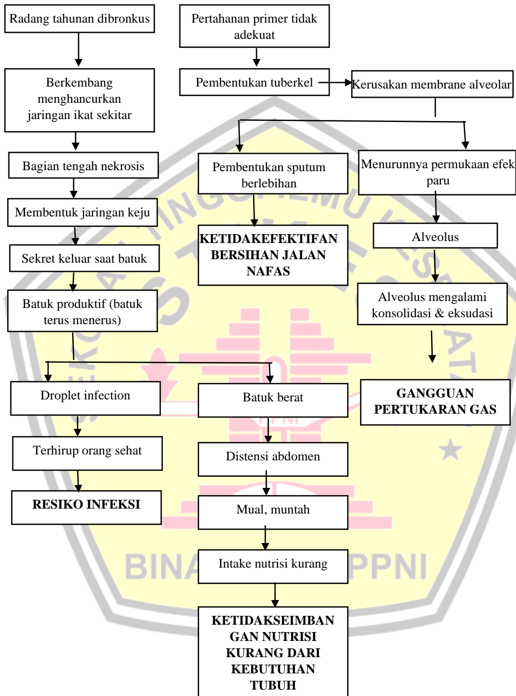
Gambar 2.1 Pathway Tuberculosis
